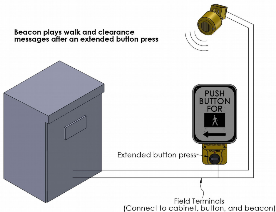
Figure 5. Beacon Connection and Activation Diagram.
