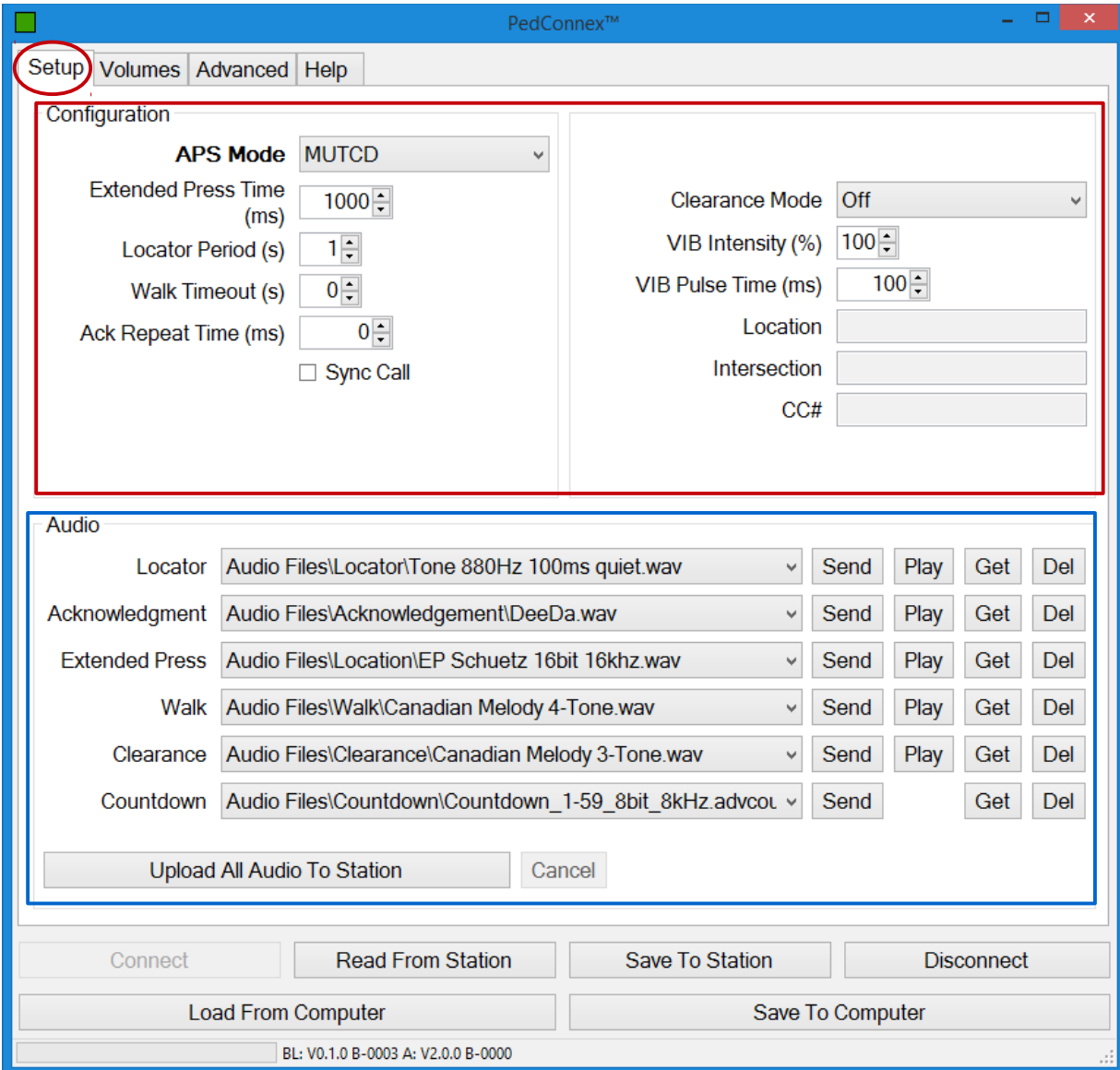
Figure 1. Setup Tab in MUTCD Mode.
