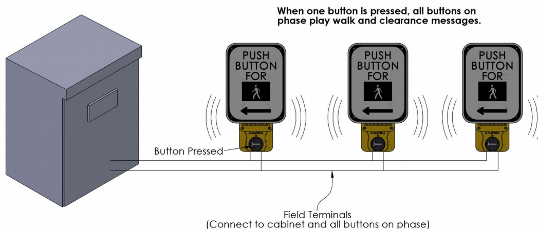
Figure 2. Sync Call Connection and Activation Diagram.
