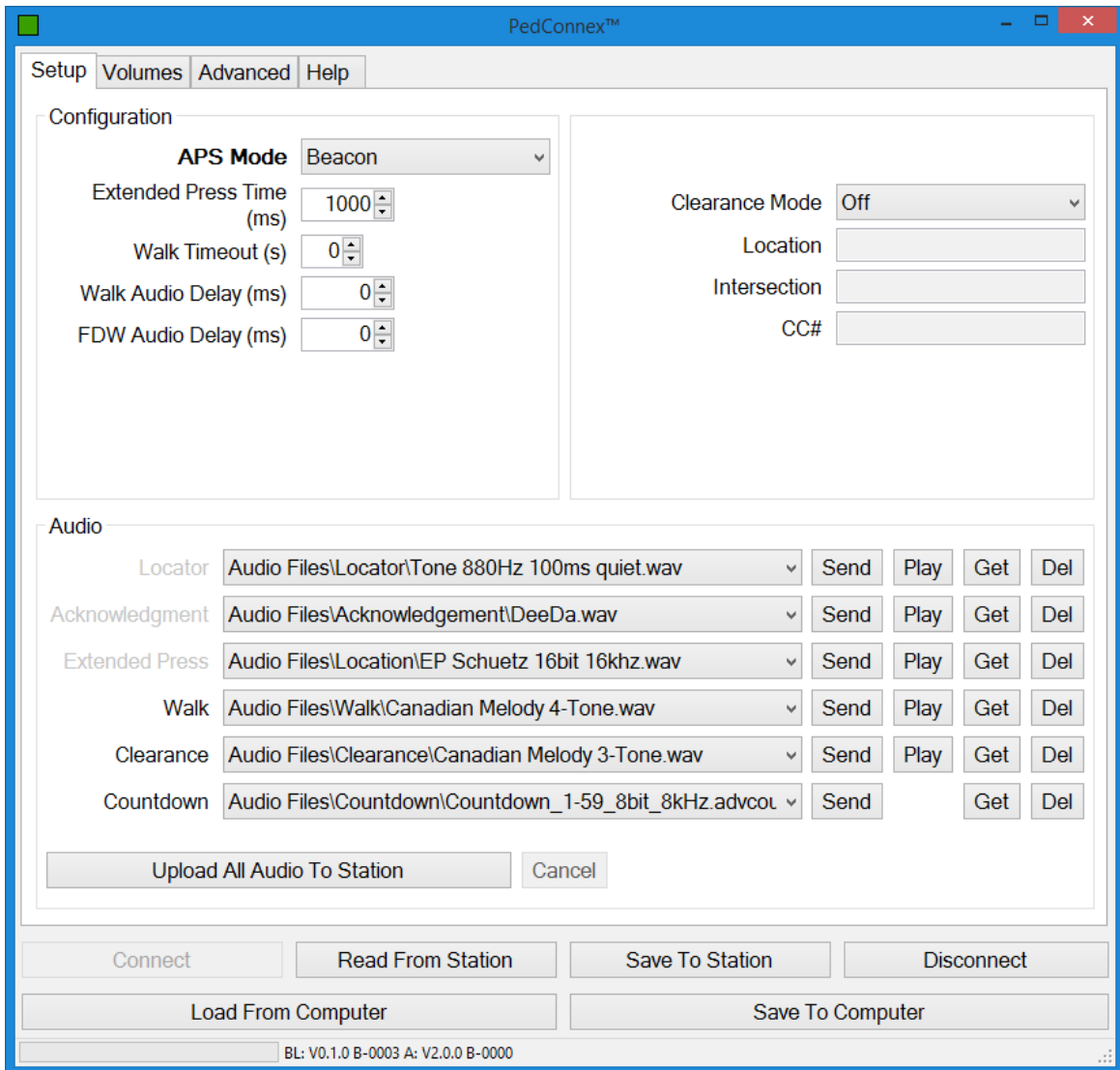
Figure 4. Setup Tab in Beacon Mode
